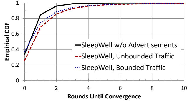
Figure 9: Adjustment rounds until a SleepWell AP reaches a converged beacon placement. 10 rounds takes \approx 3\text{s} .
