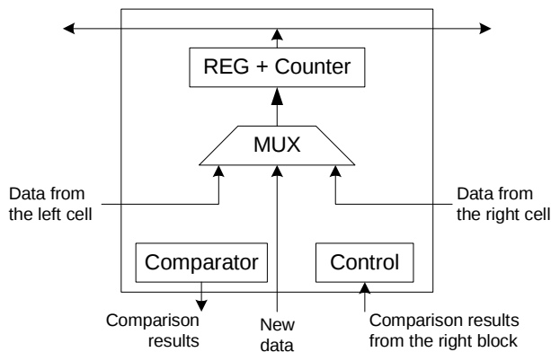
Figure 3. The PQ cell architecture.
