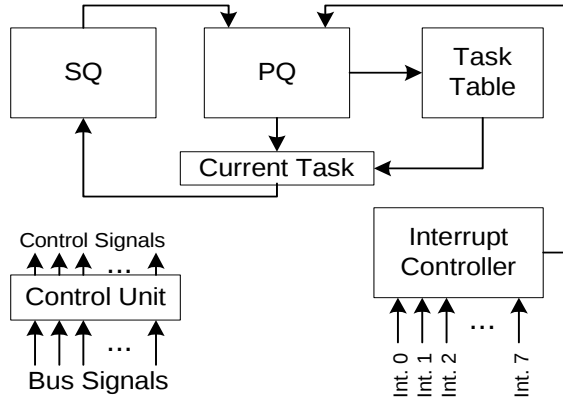
Figure 1. The configurable hardware scheduler micro-architecture.
