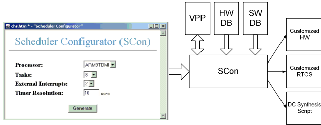
Figure 7. The Scheduler Customization Flow.
