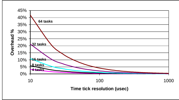
Figure 8. The scheduler and the time tick processing overheads in MicroC/OS II.
